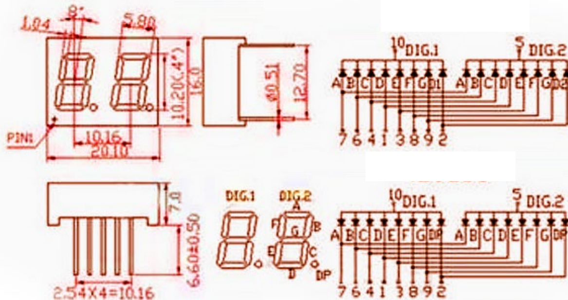
Common Anode
